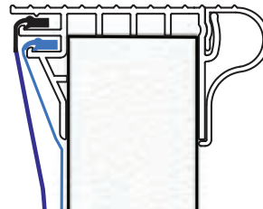
4" Coping
