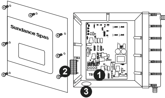
Figure C Control Box
