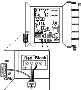
Figure D Terminal Block 240V Wire Connection
