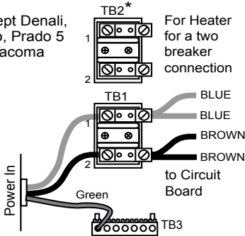
Single Breaker
