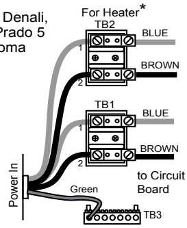
Dual Breaker
