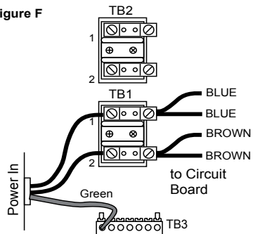
All Export Models: 230 VAC, 3-Wire (50 Hz)
