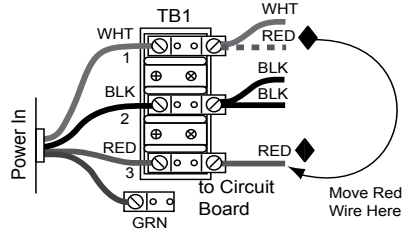
North American Denali/Tacoma Convertible Models: 240 VAC, 4-Wire Connection (60 Hz)
