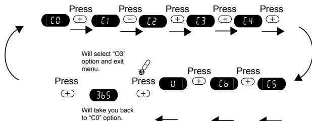
Figure 2: Menus for spas NOT equipped with a circulation pump.
