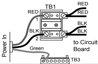
North American Models : 240 VAC, 3-Wire Connection (60 Hz)
